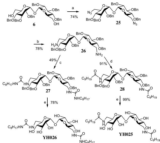
Scheme 5. Reagents: (a) (1) \text{TiF}_2\text{O} , pyr., \text{CH}_2\text{Cl}_2 ; (2) \text{NaN}_3 , DMF; (b) \text{PMe}_3 , THF, NaOH; (c) triphosgene, \text{Et}_3\text{N} , \text{C}_8\text{H}_{17}\text{NH}_2 ; (d) \text{C}_9\text{H}_{19}\text{COCl} , \text{CH}_2\text{Cl}_2 ; (e) \text{H}_2 , \text{Pd}(\text{OH})_2/\text{C} , MeOH.
