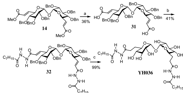
Scheme 7. Reagents: (a) \text{LiOH}-\text{H}_2\text{O} , THF, \text{H}_2\text{O} ; (b) \text{H}_2\text{NNHC}(\text{O})\text{C}_7\text{H}_{15} ; (c) \text{H}_2 , \text{Pd}(\text{OH})_2/\text{C} , MeOH.
