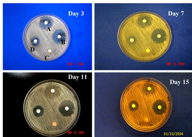
Figure 2. Assay of YH023 and INH against M. smegmatis in water/DMSO solution. A: INH (250 \mu\text{g/mL} ); B: INH (250 \mu\text{g/mL} ) + YH023 (10 mg/mL); C: DMSO; D: YH023 (10 mg/mL).
