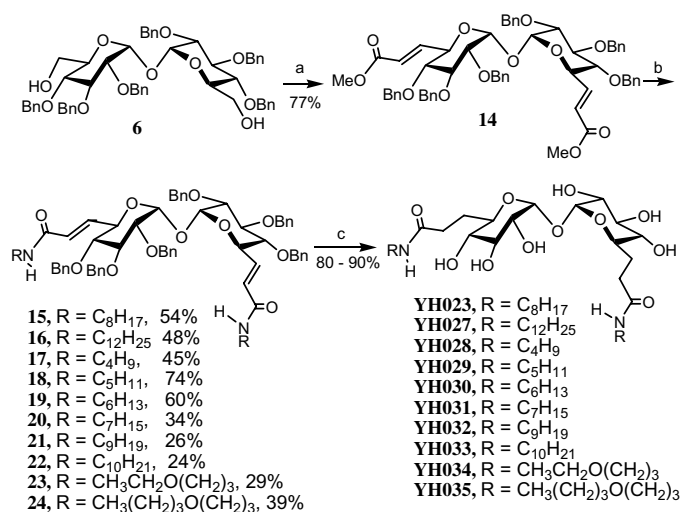
Scheme 4. Reagents: (a) (1) (COCl) 2 , DMSO, DIPEA, (2) MeOC(O)CH 2 P(O)(OEt) 2 , NaH, THF; (b) alkyl amines, AlMe 3 , CH 2 Cl 2 ; (c) H 2 , Pd(OH) 2 /C, MeOH.
