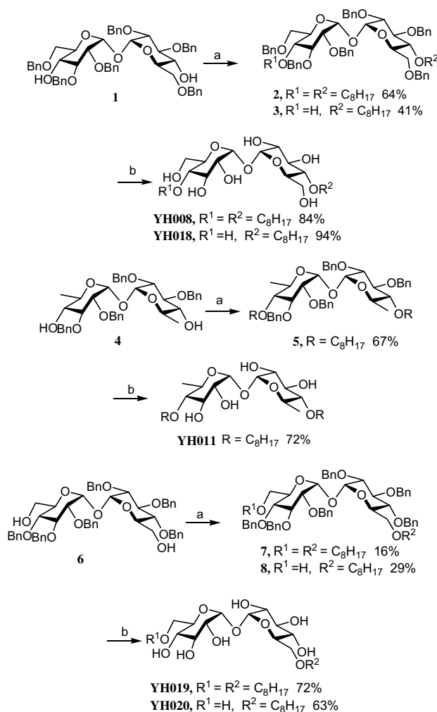
Scheme 2. Reagents: (a) C 8 H 17 Br, NaH, TBAI, THF; (b) H 2 , Pd(OH) 2 /C, MeOH.
