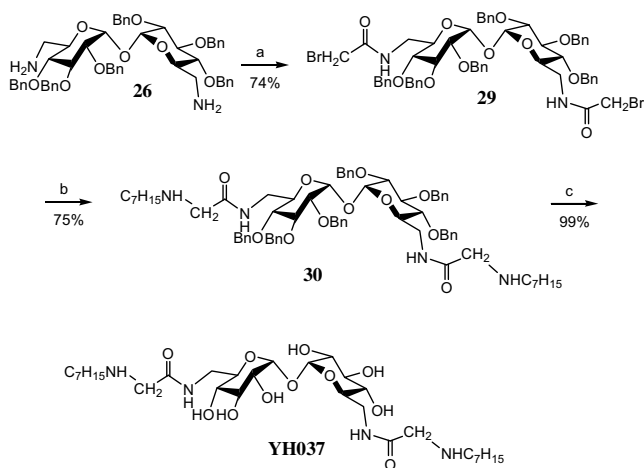
Scheme 6. Reagents: (a) \text{BrCH}_2\text{CO}_2\text{H} , DMF; DIC; (b) \text{C}_7\text{H}_{15}\text{NH}_2 , \text{Cs}_2\text{CO}_3 , DMF; (c) \text{H}_2 , \text{Pd}/\text{C} , MeOH.
